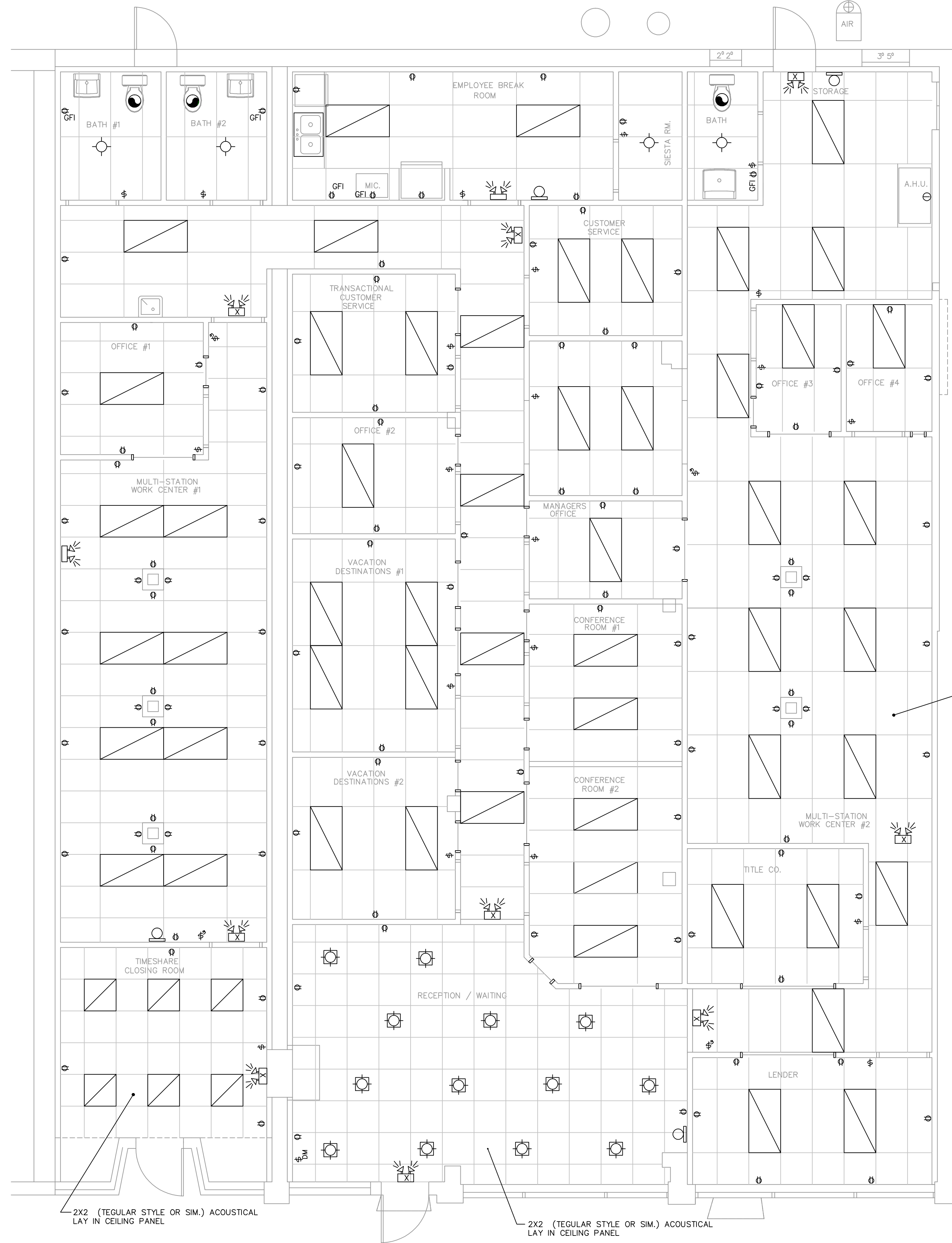
EXISTING REFLECTIVE CEILING / ELECTRICAL PLAN 1/4"=1'-0"
