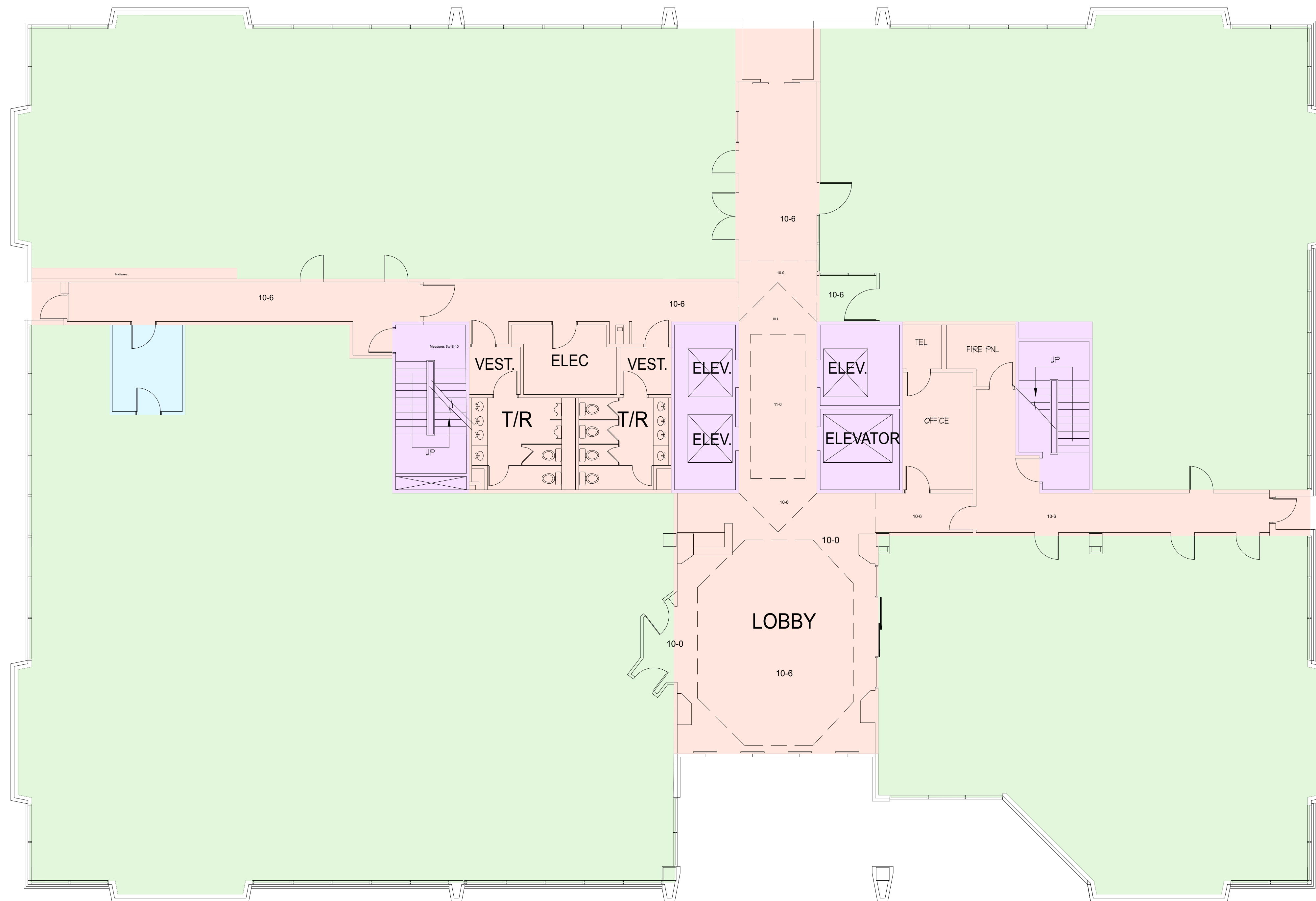
FIRST FLOOR TOWER I MEDICAL OFFICE BUILDING
